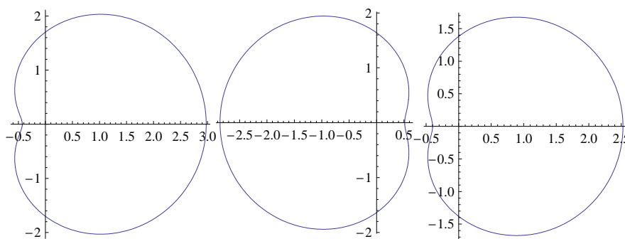
Fig. 2. The images of the unit disk by k_{p,q} for p + q = 1; p + q < 1; p + q > 1 .
