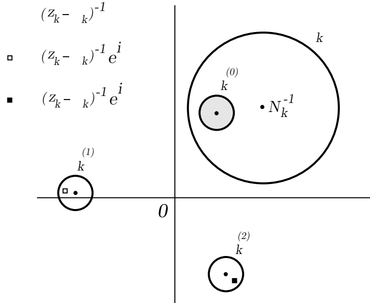
Fig. 1 Selection of a proper disk root
